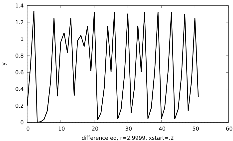
Figure 13.1: Logistic difference equation
