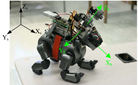
Fig. 6. (A) An unencumbered Sony AIBO robot. It has 3DOF of the head and is capable of communicating over a wireless interface with a computer. (B) The modified Sony AIBO robot. An X10® camera system mounted within a Fick gimbal system that is controlled by Servocontroller mounted on the back of the robot.
