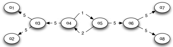
Figure 2: Weighted argument system W_1 from Example 1.
