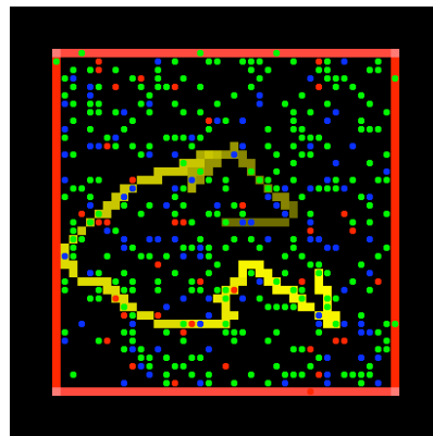
Figure 8: Gas molecules in a box. Fast particles in red, mid-speed in green and slow particles in blue. The yellow zig-zag line traces the movement of a single particle.
