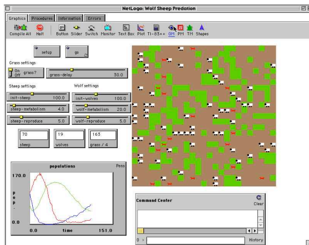
Figure 6: The NetLogo layout for the wolf-sheep predation model. In the upper left is the interface area that allows users to set model parameters and run simulations. To its right is the NetLogo graphics window that displays each individual wolf and sheep. Below the interface is a population plot window. To its right is a command center for interactively running commands.
