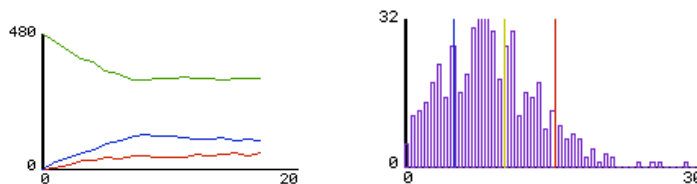
9a: plot of number of fast, medium, slow particles 9b: histogram of particle speeds
