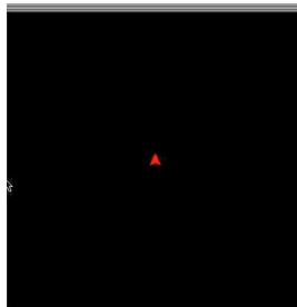
Figure 1: Create-turtles 1000
