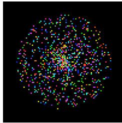
Figure 3: forward random 20
