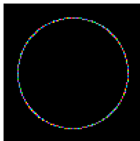
Figure 2: Forward 20
